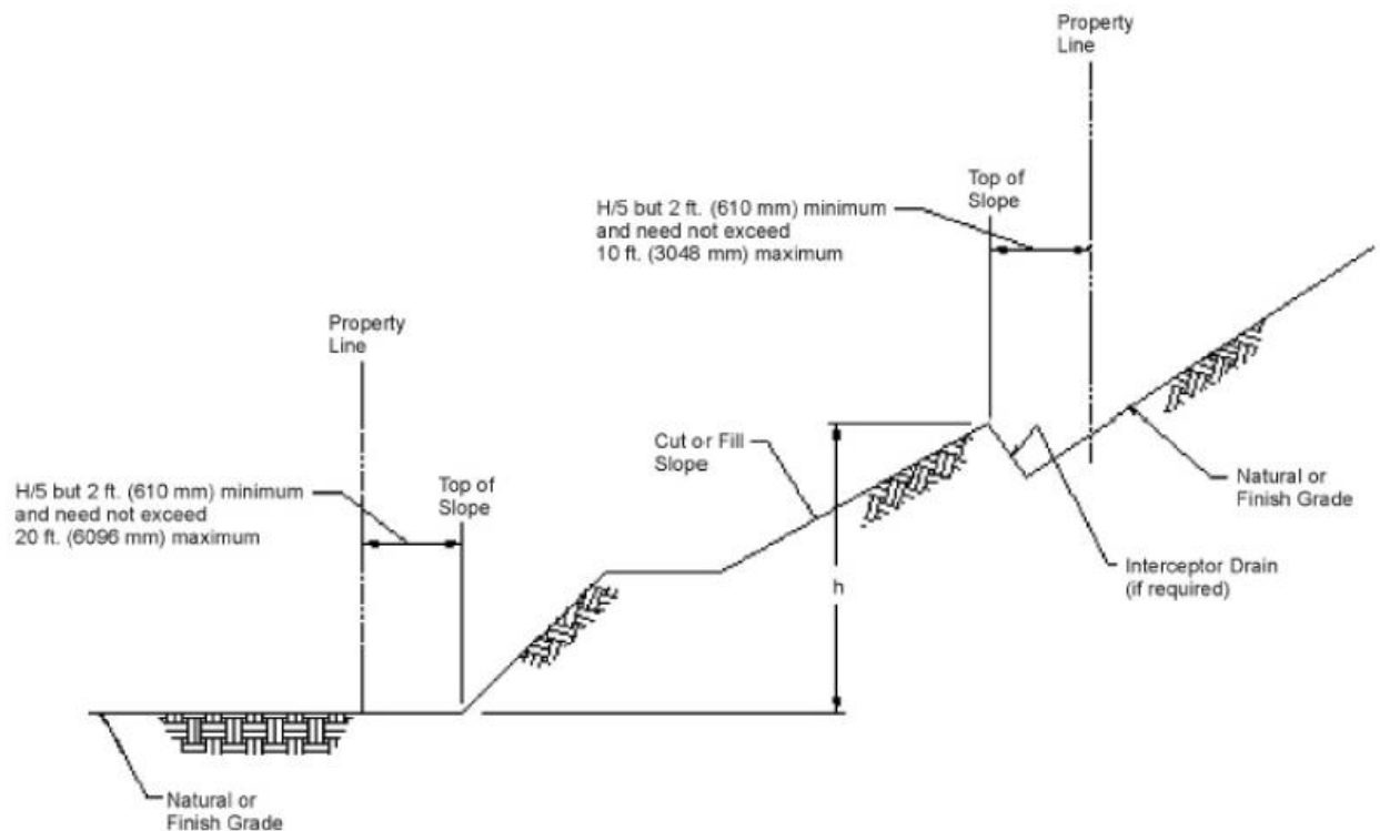
FIGURE 18.75.060 DRAINAGE DIMENSIONS
