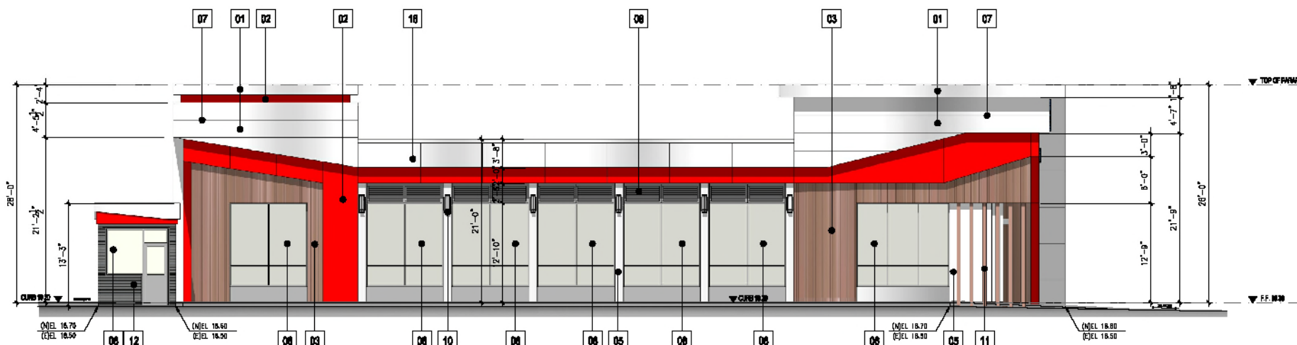
WASH TUNNEL BLDG WEST ELEVATION SCALE: 1/8" = 1'-0"
