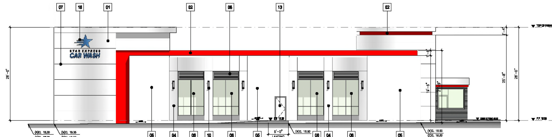
WASH TUNNEL BLDG EAST ELEVATION SCALE: 1/8" = 1'-0"
