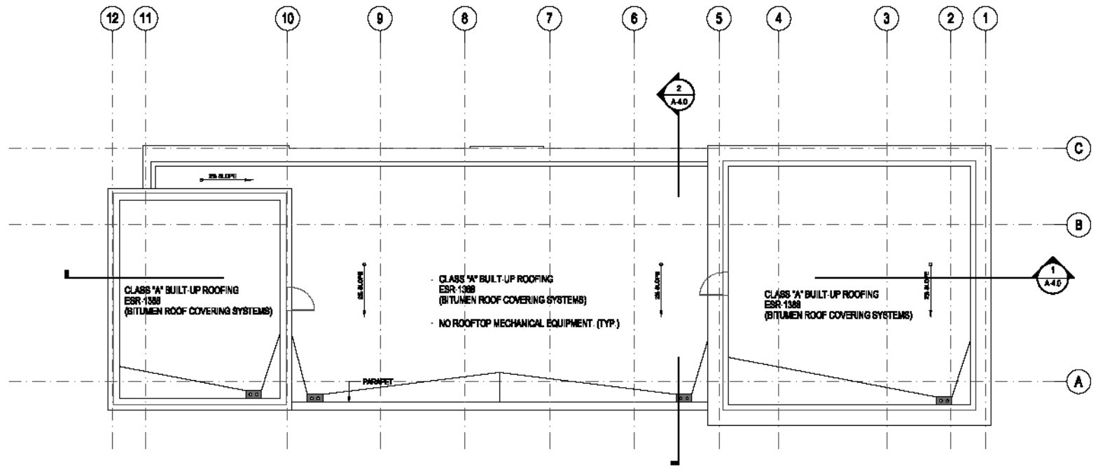
WASH TUNNEL BLDG. ROOF PLAN SCALE: 1/8" = 1'-0" 2
