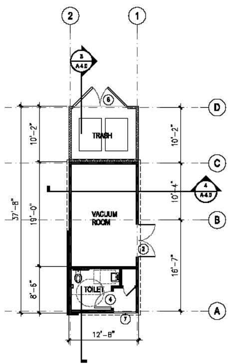
TOILET, VACUUM RM BLDG. FLOOR PLAN SCALE: 1/8" = 1'-0" 3
