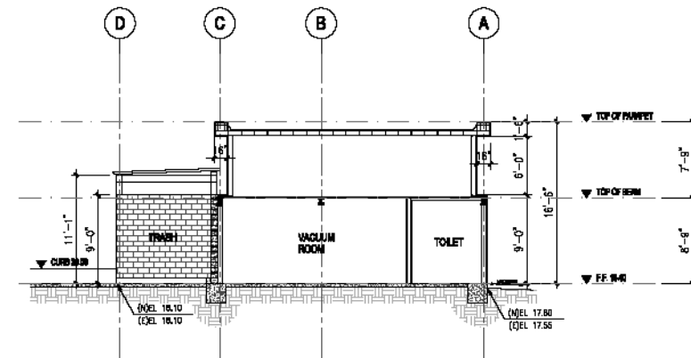
TOILET, VACUUM RM. BLDG. BLDG. CROSS SECTION 3 SCALE: 1/8" = 1'-0"
