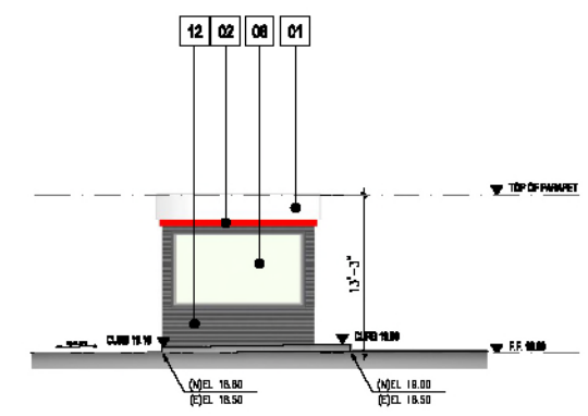
MONITORING RM. BLDG SOUTH ELEVATION SCALE: 1/8" = 1'-0" 7
