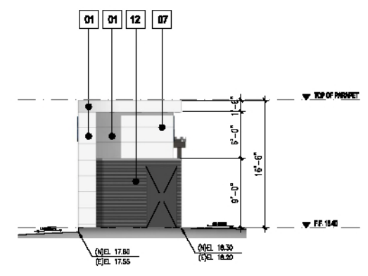
TOILET, VACUUM RM. BLDG SOUTH ELEVATION SCALE: 1/8" = 1'-0" 3
