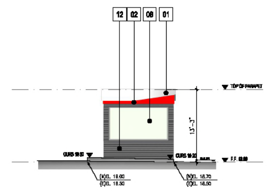
MONITORING RM. BLDG NORTH ELEVATION SCALE: 1/8" = 1'-0" 8
