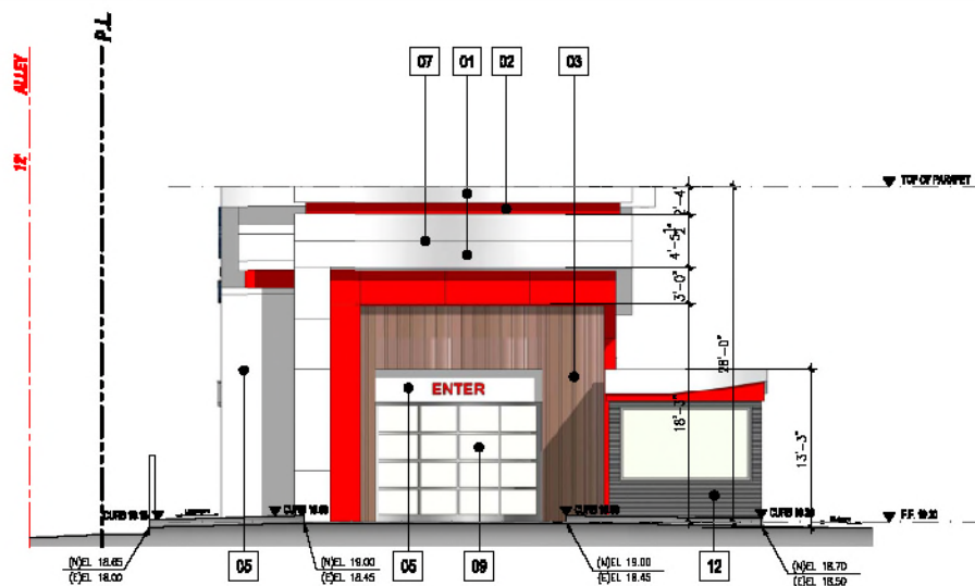
WASH TUNNEL BLDG NORTH ELEVATION SCALE: 1/8" = 1'-0"
