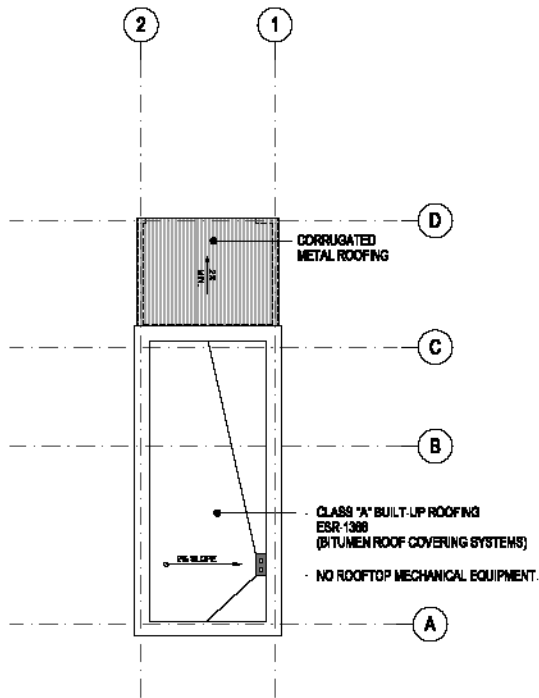
TOILET, VACUUM RM BLDG. ROOF PLAN SCALE: 1/8" = 1'-0" 4
