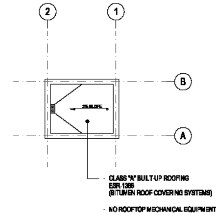
MONITORING RM. ROOF PLAN SCALE: 1/8" = 1'-0" 6
