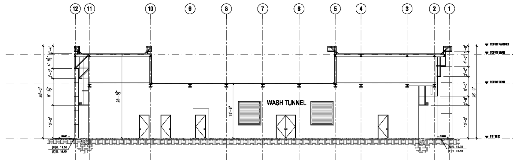
WASH TUNNEL BLDG. BLDG. CROSS SECTION 1 SCALE: 1/8" = 1'-0"
