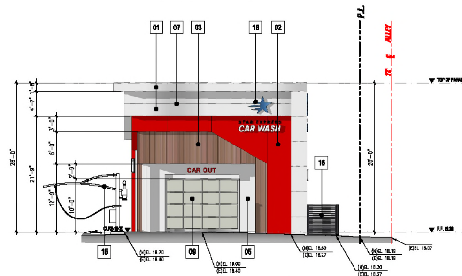
WASH TUNNEL BLDG SOUTH ELEVATION SCALE: 1/8" = 1'-0"
