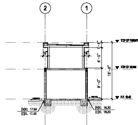
TOILET, VACUUM RM. BLDG. BLDG. CROSS SECTION 4 SCALE: 1/8" = 1'-0"
