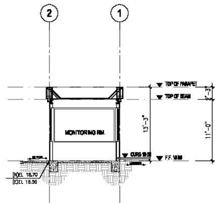
MONITORING RM. BLDG. BLDG. CROSS SECTION 6 SCALE: 1/8" = 1'-0"
