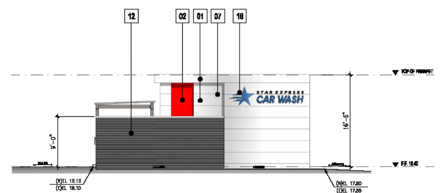
TOILET, VACUUM RM. BLDG WEST ELEVATION SCALE: 1/8" = 1'-0" 1
