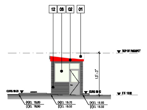
MONITORING RM. BLDG WEST ELEVATION SCALE: 1/8" = 1'-0" 6
