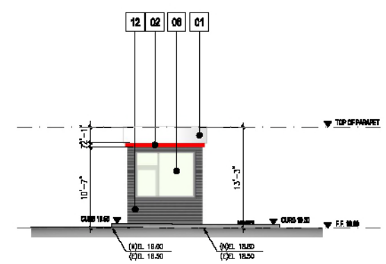
MONITORING RM. BLDG EAST ELEVATION SCALE: 1/8" = 1'-0" 5
