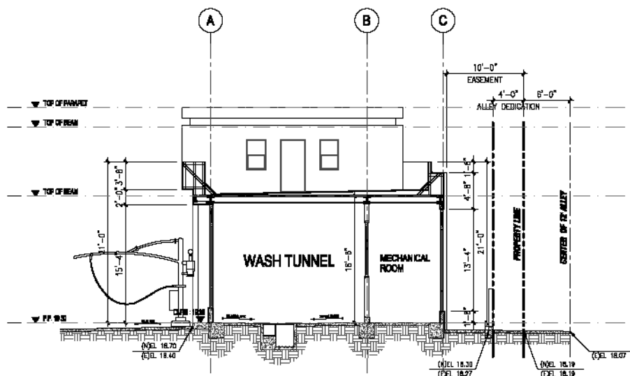
WASH TUNNEL BLDG. BLDG. CROSS SECTION 2 SCALE: 1/8" = 1'-0"
