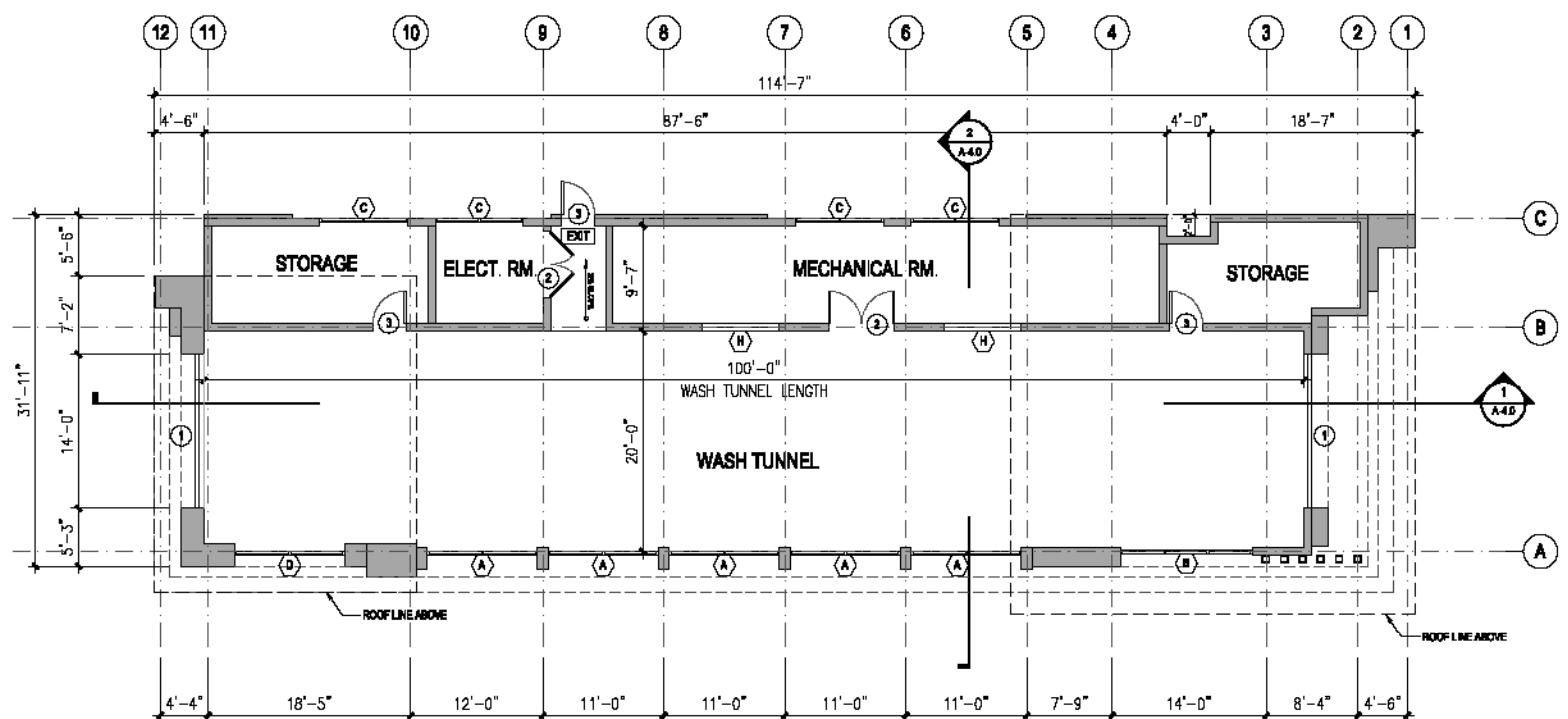
WASH TUNNEL BLDG. FLOOR PLAN SCALE: 1/8" = 1'-0" 1
