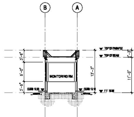
MONITORING RM. BLDG. BLDG. CROSS SECTION 5 SCALE: 1/8" = 1'-0"
