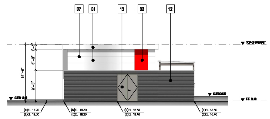
TOILET, VACUUM RM. BLDG EAST ELEVATION SCALE: 1/8" = 1'-0" 2
