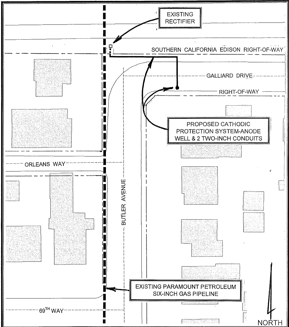
VICINITY MAP LOCATION OF A PROPOSED CATHODIC PROTECTION SYSTEM FOR AN EXISTING SIX-INCH GAS PIPELINE PROPOSED FACILITY/PIPELINE PERMIT SUPPLEMENT NO. S-2-10 UNDER FACILITY/PIPELINE PERMIT NO. P-141-83 TO PARAMOUNT PETROLEUM CORPORATION
