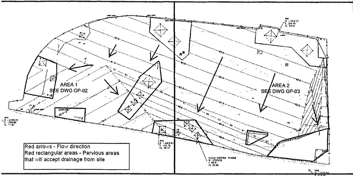
GRADING PLAN AND DRAINAGE FLOW DIRECTION
