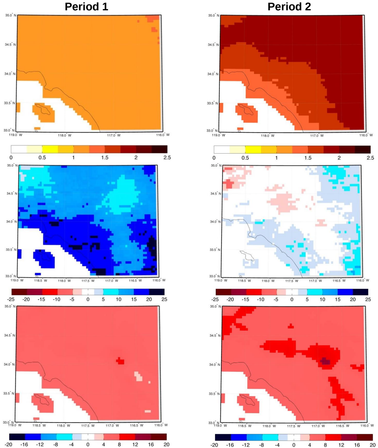
Figure 11: Ensemble average a) daily temperature changes (°C), b) daily cumulative annual precipitation percent change and c) bias corrected annual ETo percent change by Period 1 (2030) and Period 2 (2050) from baseline to RCP 8.5 for the greater Los Angeles region.
