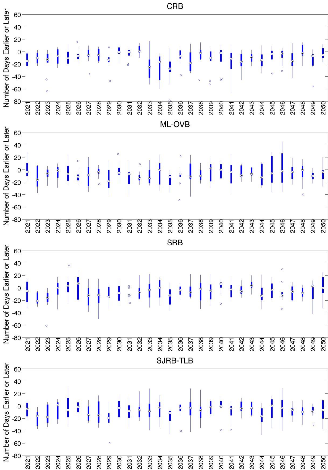
Figure 8: Change in CMD on a basin level for a) CRB, b) ML-OVB, c) SRB and d) SJRB-TLB. Boxplots represent the change of each model (n=10) under RCP 8.5 from baseline average CMDs. Black dots depict ensemble median and outliers are defined as being +/- 2.7 standard deviations from the median.
