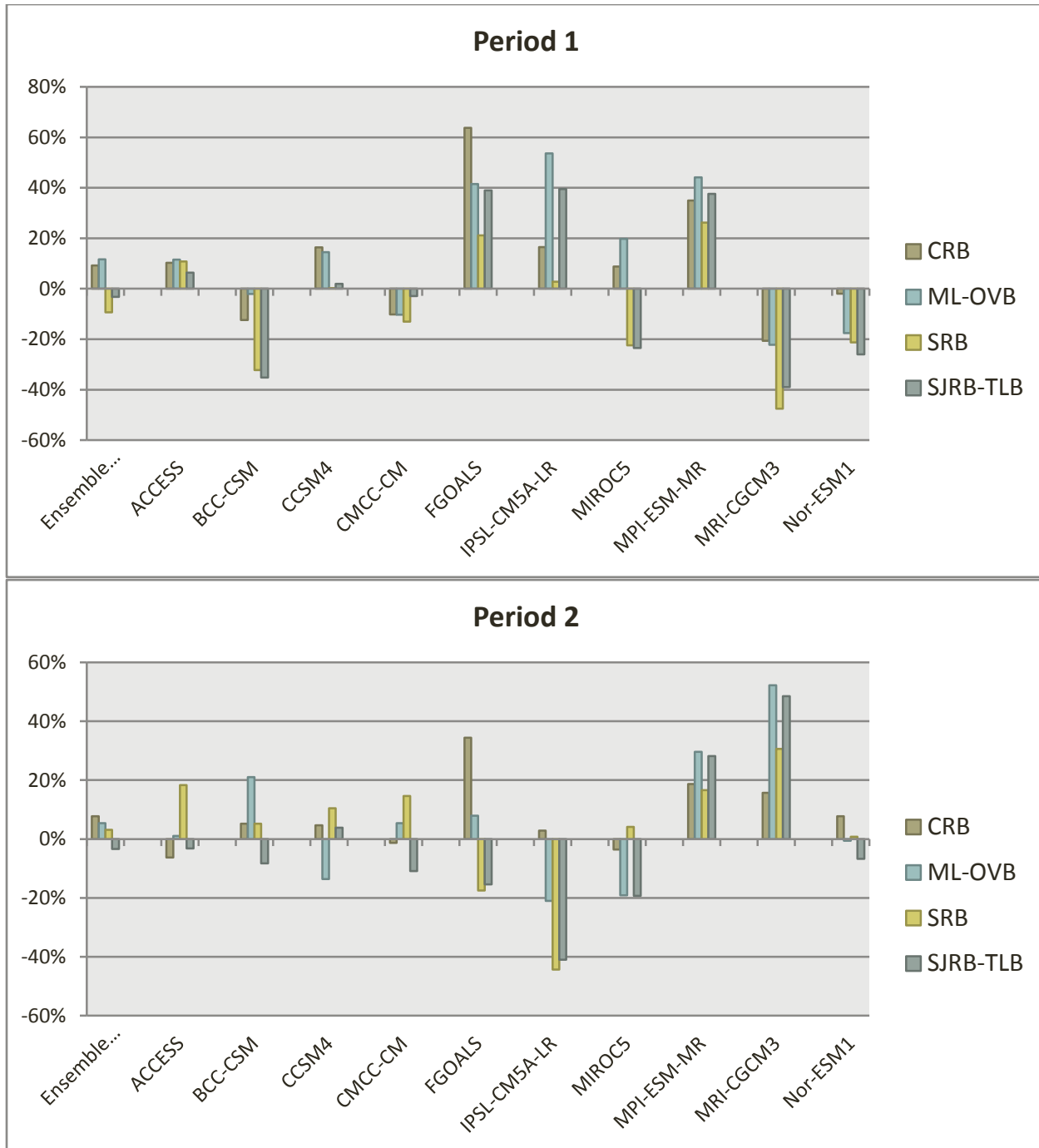
Figure 6: Ensemble and individual model average annual runoff percent changes for each basin from baseline to 2030 and 2050.
