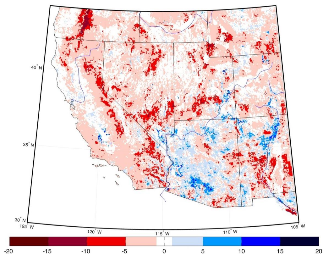
Figure 7: Change in CMD calculated for water years on a grid point basis. Negative values indicate peak runoff occurring earlier in the year as seen throughout the higher mountain ranges and the Sierra Nevada
