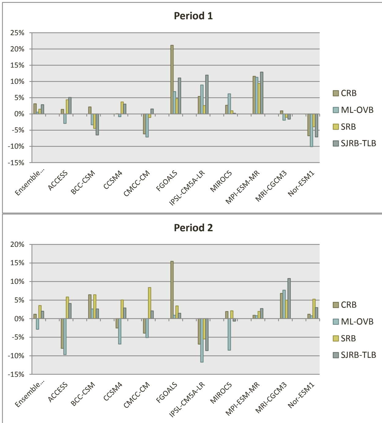
Figure 5: Ensemble and individual model average annual evaporation percent changes for each basin from baseline to 2030 and 2050.
