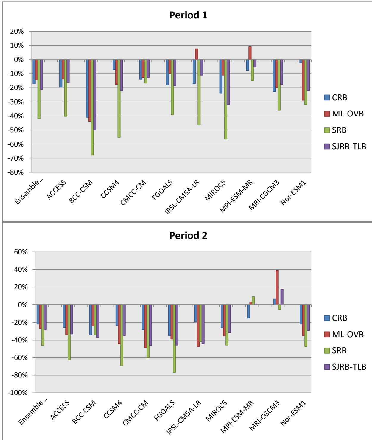
Figure 3: Ensemble and individual model average daily JFMA snow depth percent changes for each basin from baseline to 2030 and 2050.
