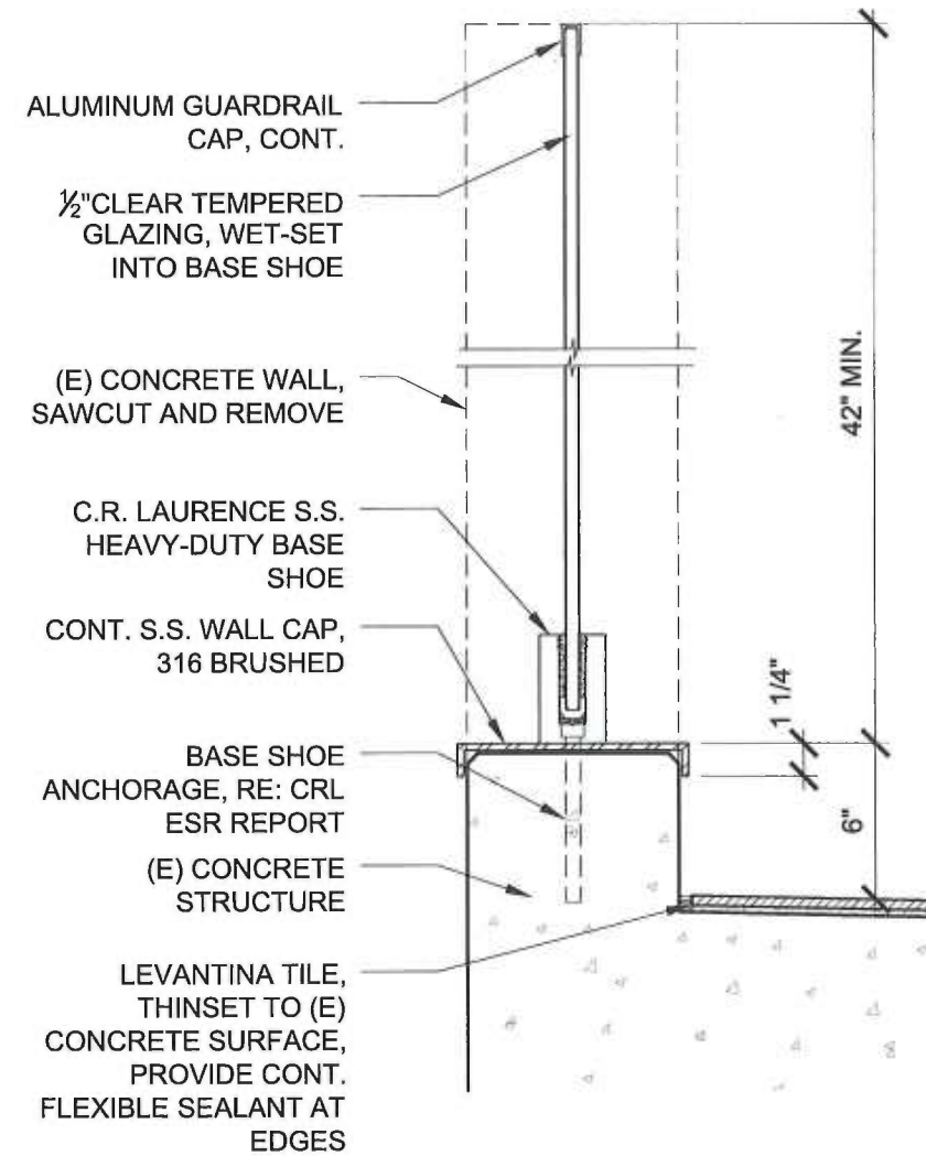
2. GLASS GUARDRAIL, TYP.
