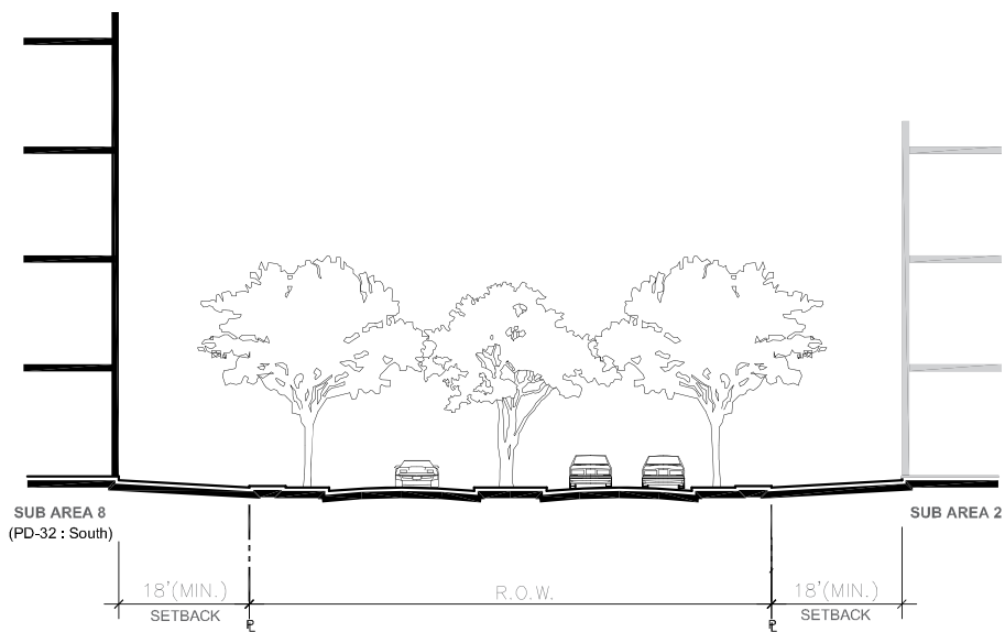
Figure 15 : Section P-P
