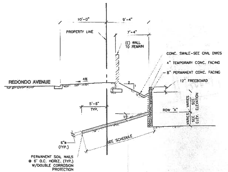
SECTION 4 3/16" = 1'-0" RW-5
