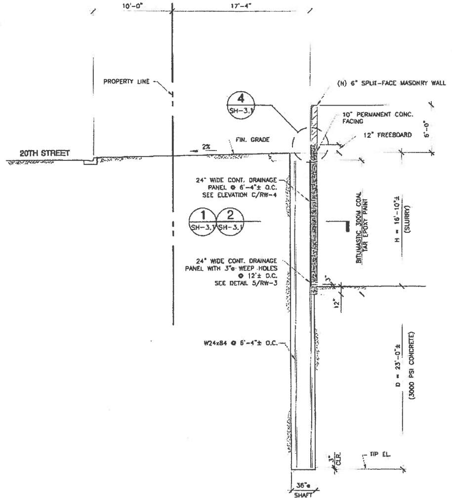
SECTION 5 3/16" = 1'-0" RW-5
