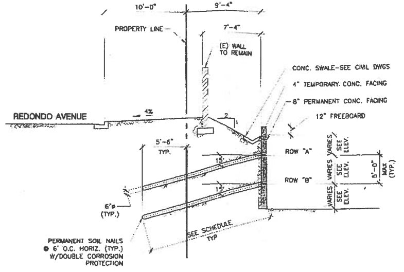
SECTION 3 3/16" = 1'-0" RW-5
