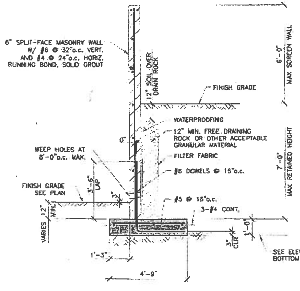
SECTION 6 3/8" = 1'-0" RW-5
