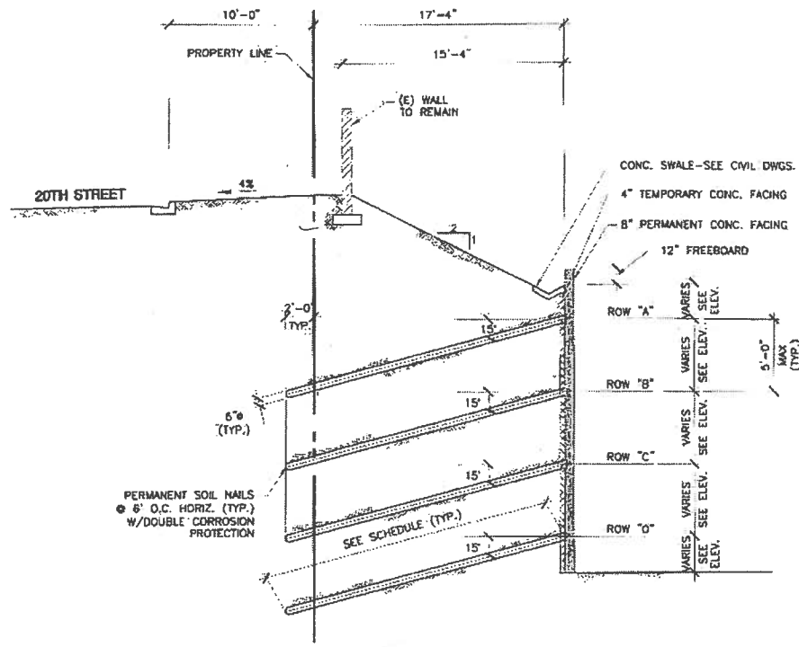
SECTION 1 3/16" = 1'-0" RW-5
