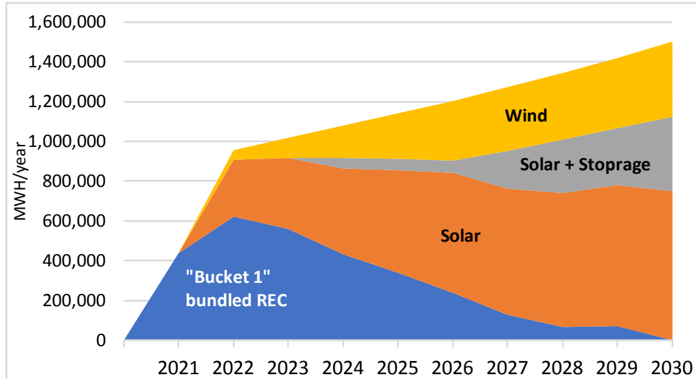
Figure 8. Renewable Power Generation by Source (Supply Scenario 1)
