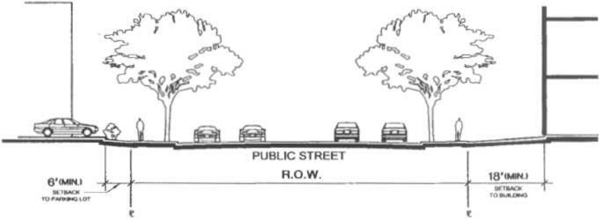
Figure 17 : Section F-F
