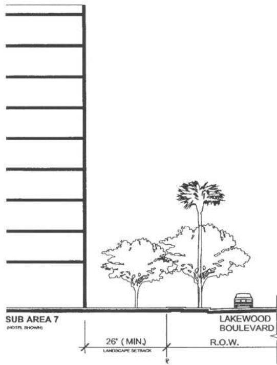
Figure 12 : Section Q-Q
