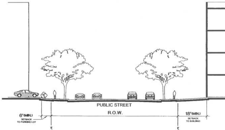
Figure 17 : Section S-S
