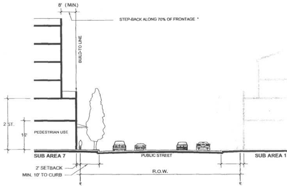
Figure 14 : Section A-A
