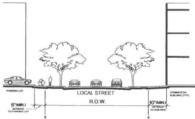
Figure 18 : Section T-T
