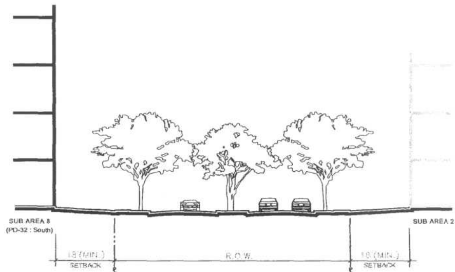
Figure 15 : Section P-P
