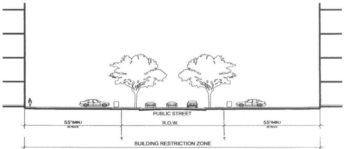
Figure 13 : Section R-R
