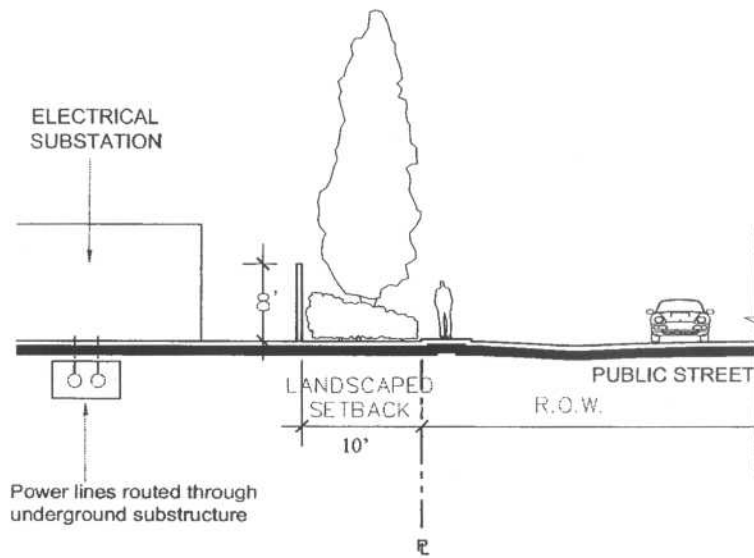
Figure 20 : Section H-H
