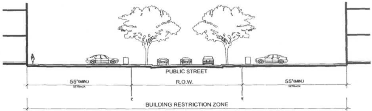
Figure 21 : Section I-I
