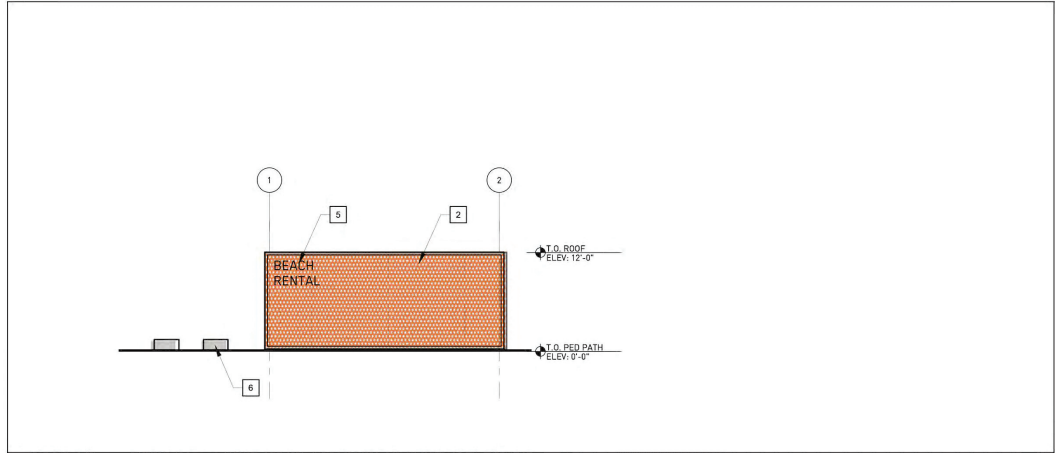
D10 A2.10 SW ELEVATION - BUILDING [B] & [C] SCALE: 1/8"=1'-0" Ref: A1.12 -
