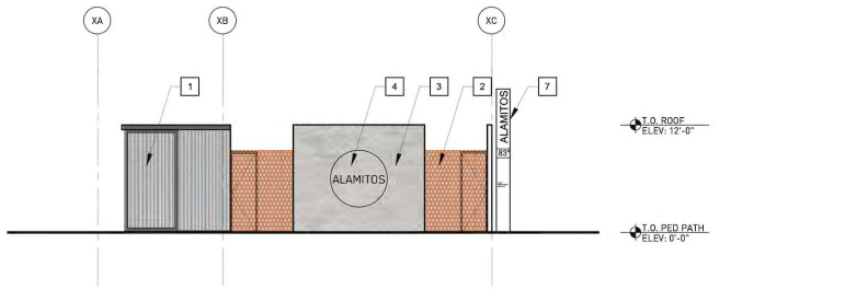
SW ELEVATION - BUILDING [B] & [C]
