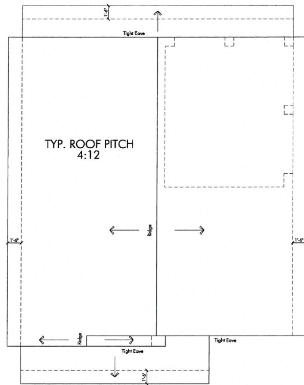
PLAN 2 SPANISH BUNGALOW ELEVATION
