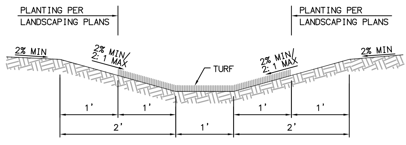
DETAIL CROSS-SECTION BIOSWALE
