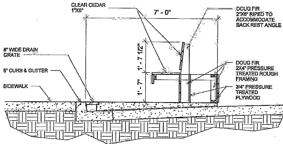
3 SECTION ACROSS PLANTER
