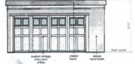
Existing Garage North Elevation
