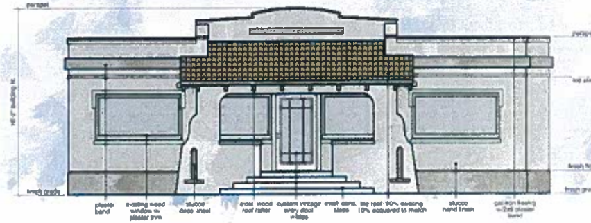
North-Street Elevation
