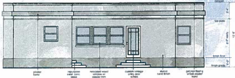
South-Rear Elevation
