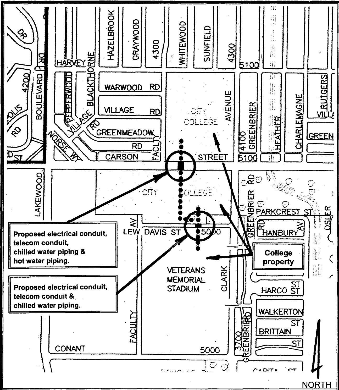
VICINITY MAP Long Beach Community College District Proposed Facility/Pipeline Permit No. P-213-05 to Allow the Installation of Conduits and Piping in City Streets
