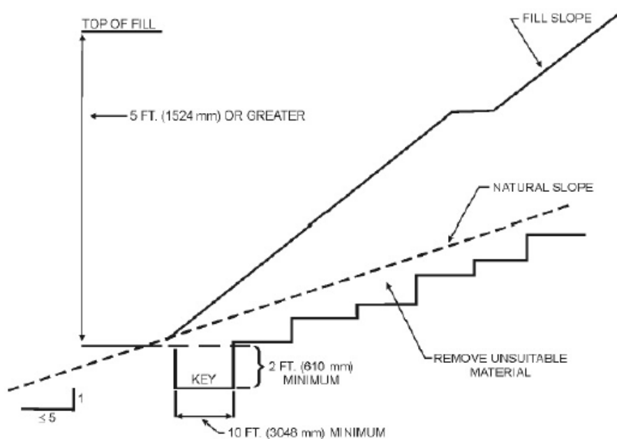
FIGURE 18.75.050 BENCHING DETAILS
