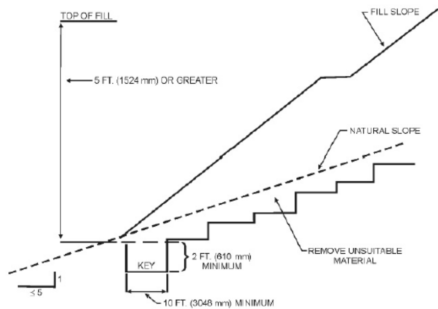
FIGURE 18.75.050 BENCHING DETAILS
