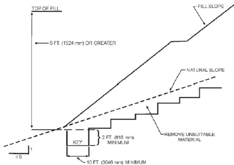
FIGURE 18.75.050 BENCHING DETAILS
