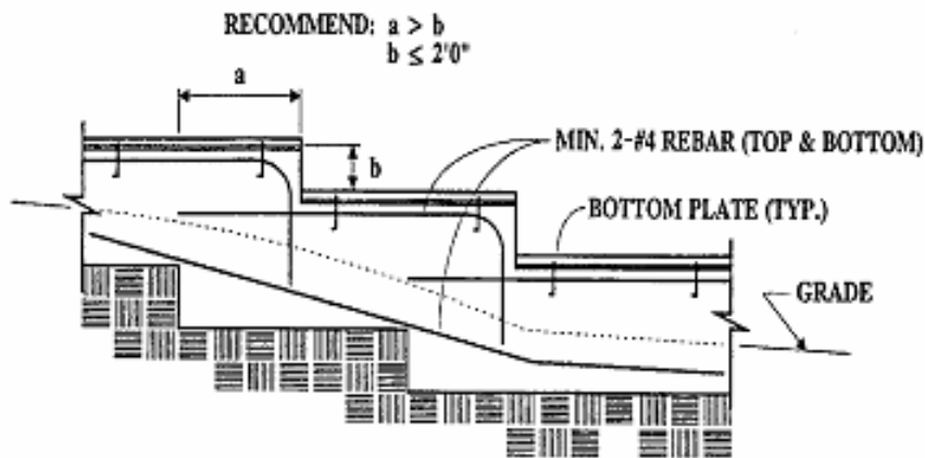
STEPPED FOUNDATIONS
