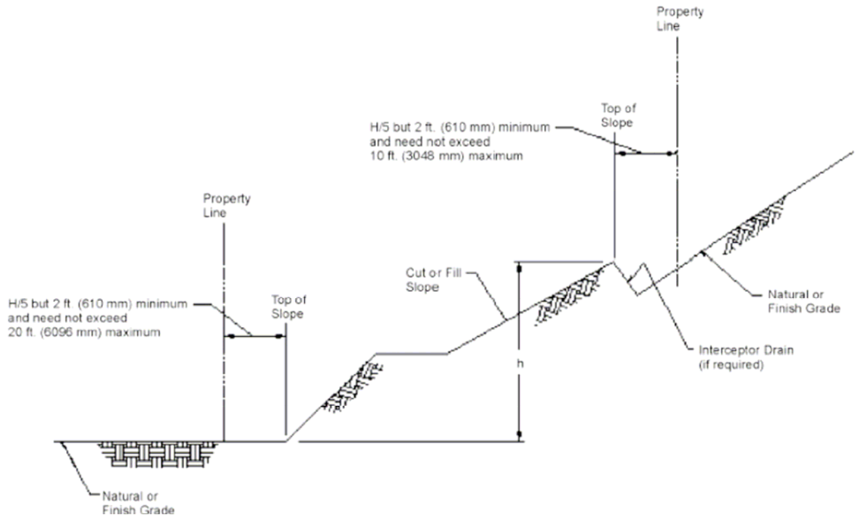
FIGURE 18.75.060 DRAINAGE DIMENSIONS
