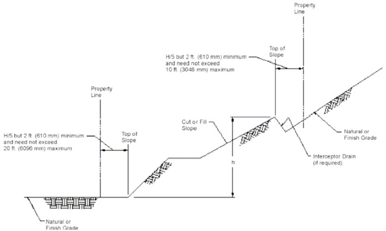
FIGURE 18.75.060 DRAINAGE DIMENSIONS
