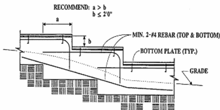
STEPPED FOUNDATIONS
