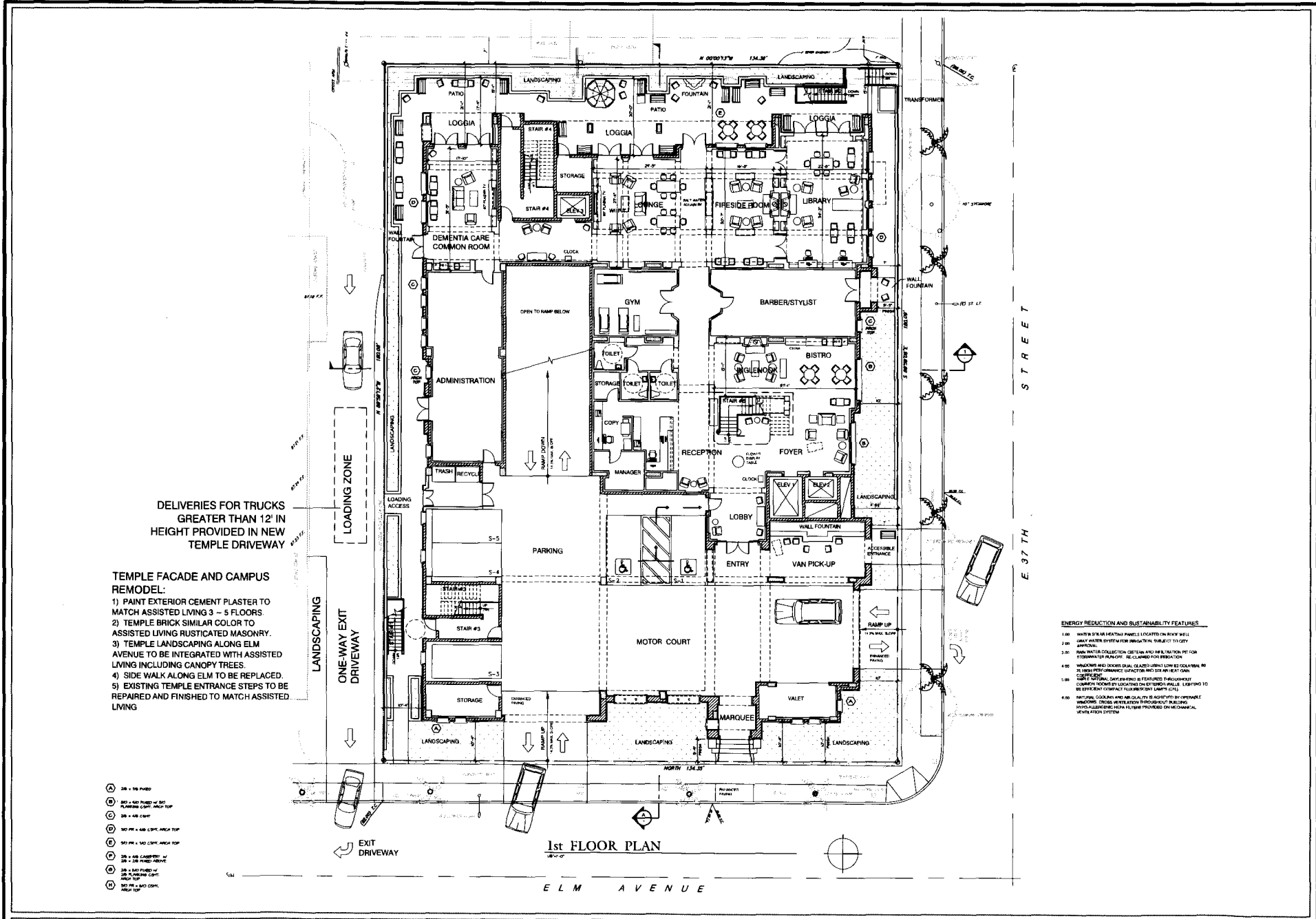
Figure IV.C-15 First Floor Plan
