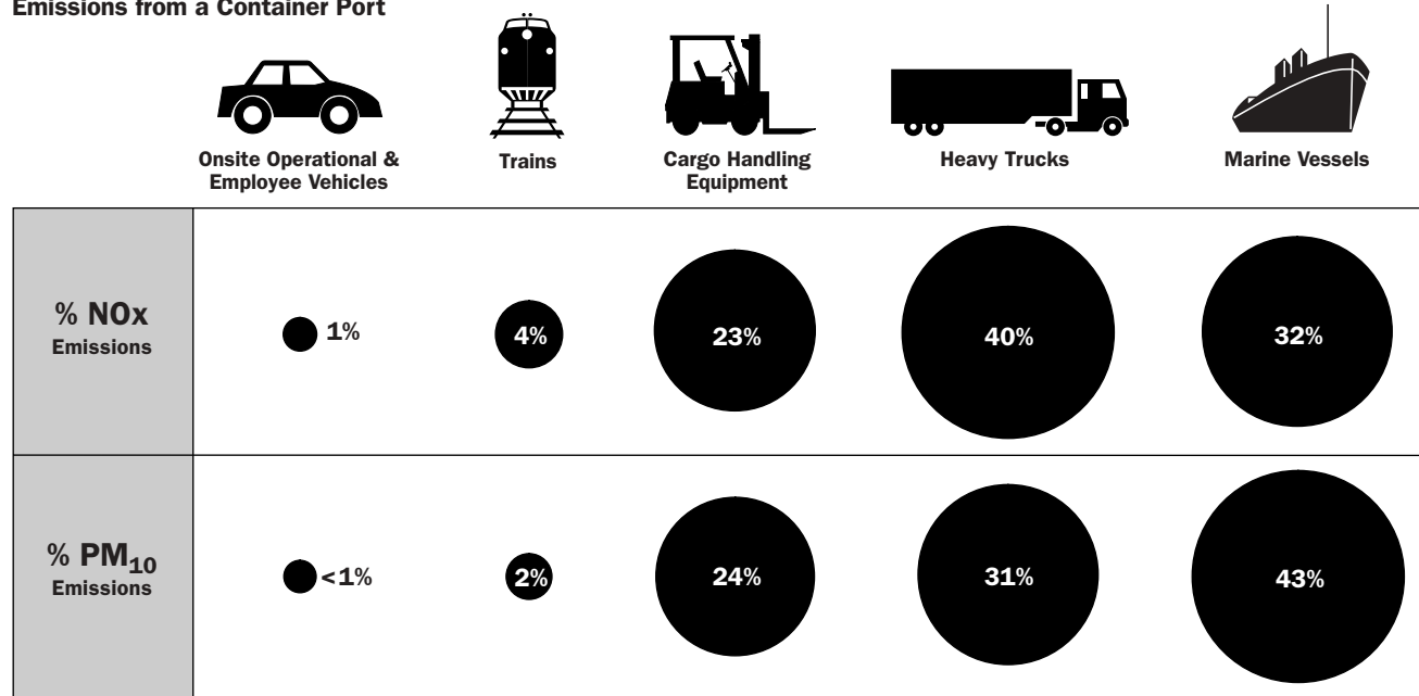
FIGURE 1 Average Contributions of Various Port-Related Sources to Total Nitrous Oxide (NOx) and Particulate Matter (PM 10 ) Emissions from a Container Port
